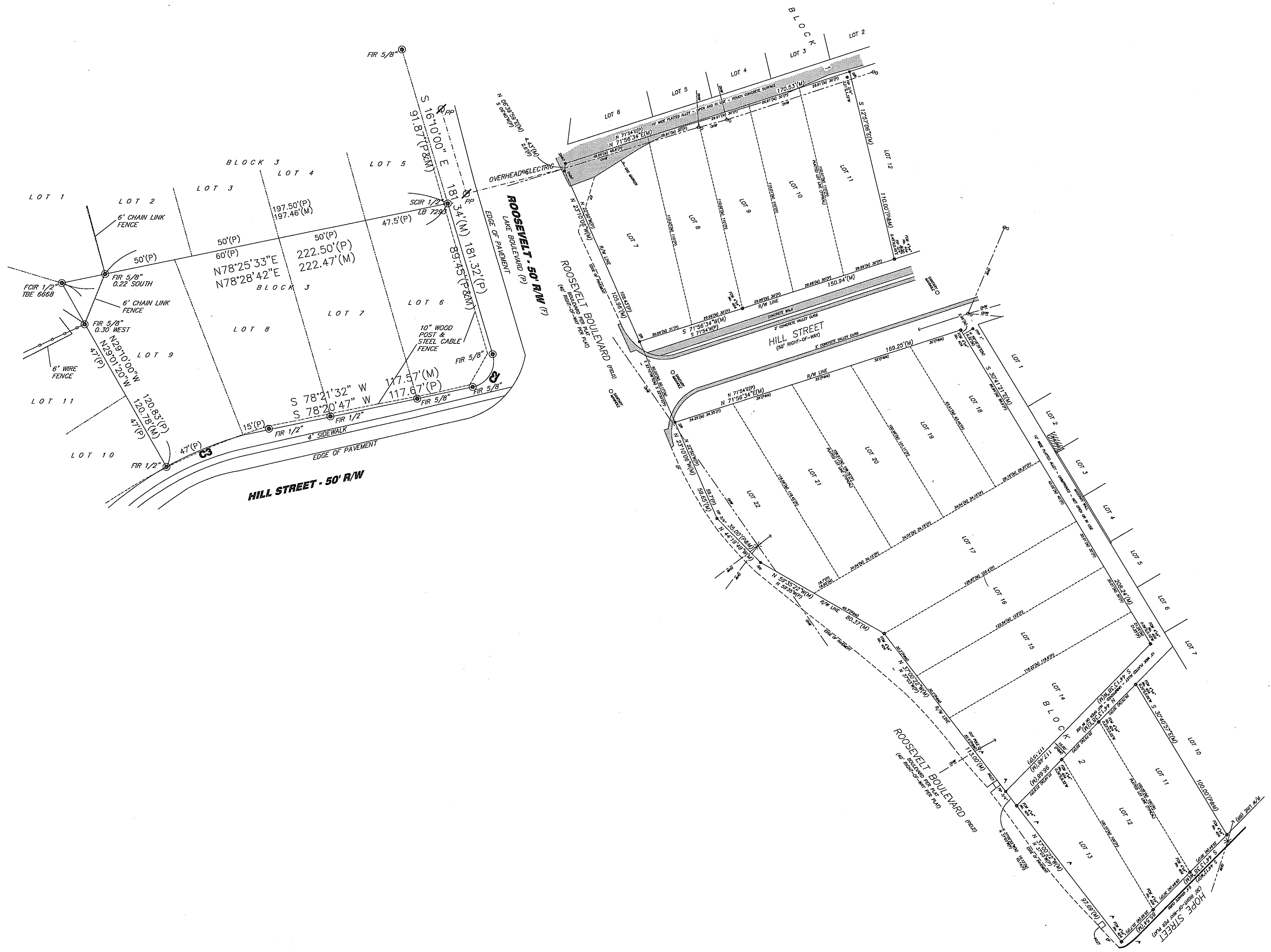
↑ N SITE PLAN 1" = 30'
